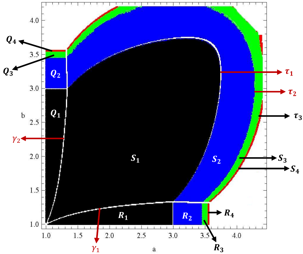
Figure 9. The bifurcation scenario of a fixed point of the competition logistic model in the parameter space (a, b)
