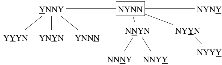
Fig. 1. A 2-quasiball in the hypercube Q_4 satisfying Definition 17 is given a tree structure with stem NYNN. A child agrees with its parent before the underlined position, is opposite at the underlined position, and has unconstrained relationship with its parent afterward.
